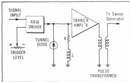
Fig. 8. Basic trigger circuit used in hp-175A Oscilloscope.
