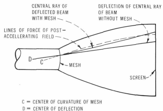
Fig. 2. Diagram indicating how spherical shield or mesh in new crt terminates post-acceleration lines of force so as to magnify beam deflection angle.
