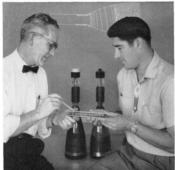
Fig. 11. Gun and deflection plate assembly used in new crt is discussed by William Kruger, tube designer and -hp- manager of crt development, and Floyd Siegel, project leader for Model 175A Oscilloscope.
