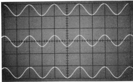
Fig. 3. Oscilloscope illustrating freedom of new -hp- crt from deflection defocusing of trace. Oscilloscope is triple exposure with trace moved to new vertical position between exposures. This and other oscillograms herein also indicate how increased vertical scan of 6 cm is especially valuable when more than one trace is used.
